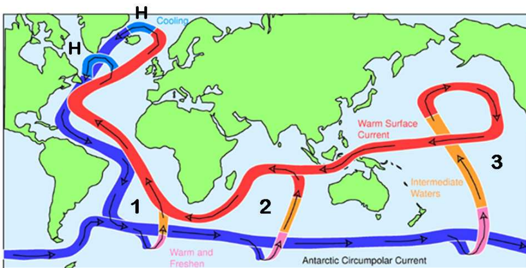
Figure 5. Idealized new estimate of the deep water Global Ocean Conveyor Belt showing the typical locations in the Southern Hemisphere of the required return cold upwelling circulation (areas 1, 2, 3) to balance the North Atlantic thermohaline ocean subsidence (H areas). Figure courtesy of John Marshall, of MIT.
