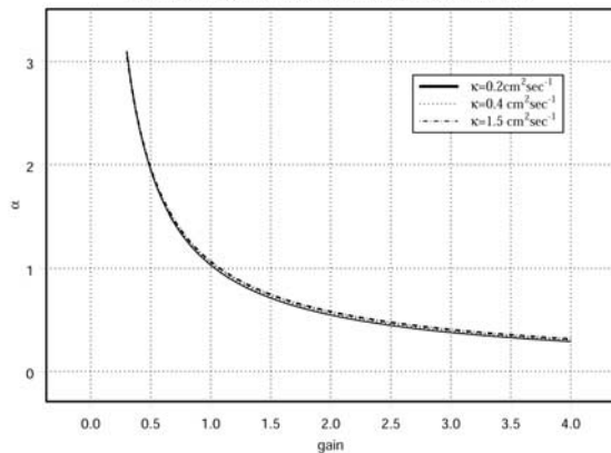
Factor by which forcing is multiplied in order to match observations as a function of gain for different choices of thermocline diffusivity
