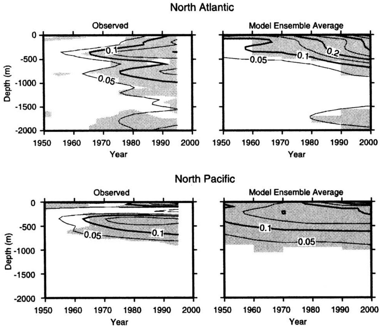
Figure 1. Modeled and observed temporal and vertical changes in the temperature in the upper 2000 m of the data-rich North Pacific and North Atlantic Oceans. Near the surface, where interannual and decadal changes and external forcings strongly affect the thermal structure, any agreement is largely due to chance. Gray-shaded regions denote areas where changes are statistically different from zero. The model broadly reproduces the main features of the vertical structure and its temporal evolution over the last 40 years. The contour interval is 0.05^{\circ}\text{C} . From Barnett et al. [2001].
