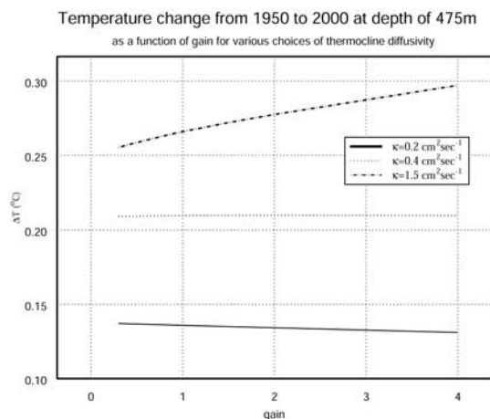
Figure 3. Calculated ocean temperature change between 1950 and 2000 at a depth of 475 m as a function of gain (climate sensitivity) for various choices of thermocline diffusivity.
